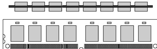
Double Sided DIMM
